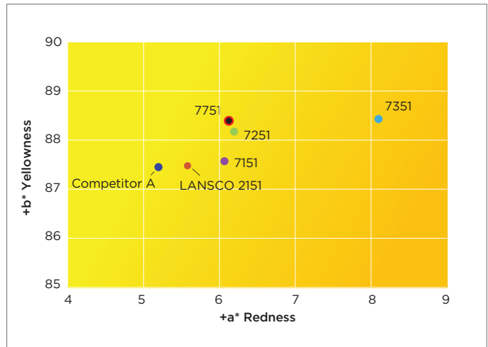
TINT COLOUR CHANGE ON WEATHERING EXPOSURE FOR PY.151 GRADES
