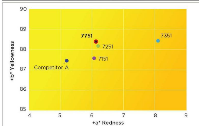
MASSTONE COLOR CHART SHOWING PIGMENT YELLOW 151 GRADES
