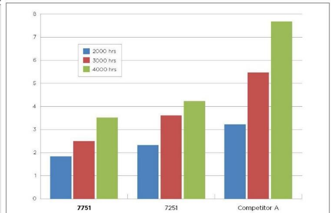
TINT COLOR CHANGE ON WEATHERING EXPOSURE FOR PY.151 GRADES
